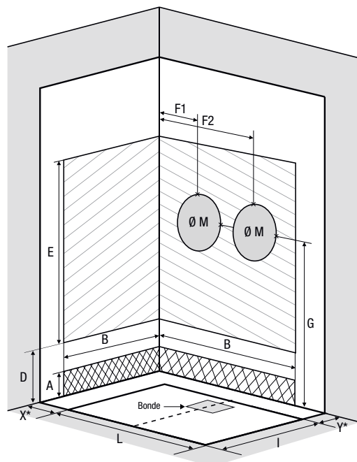
Kinemagic Royal+ / Royal
